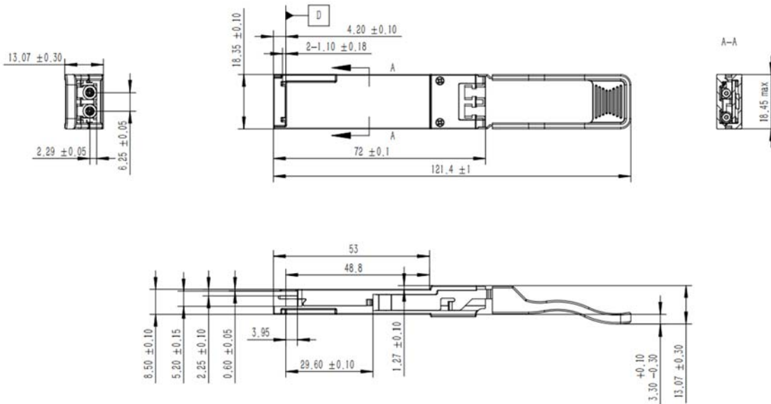
Figure 2. Mechanical dimensions
